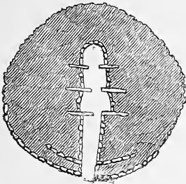
No. 3. Cairn at Yarhouse, opened by Mr. RHIND. Scale \frac{1}{360}
